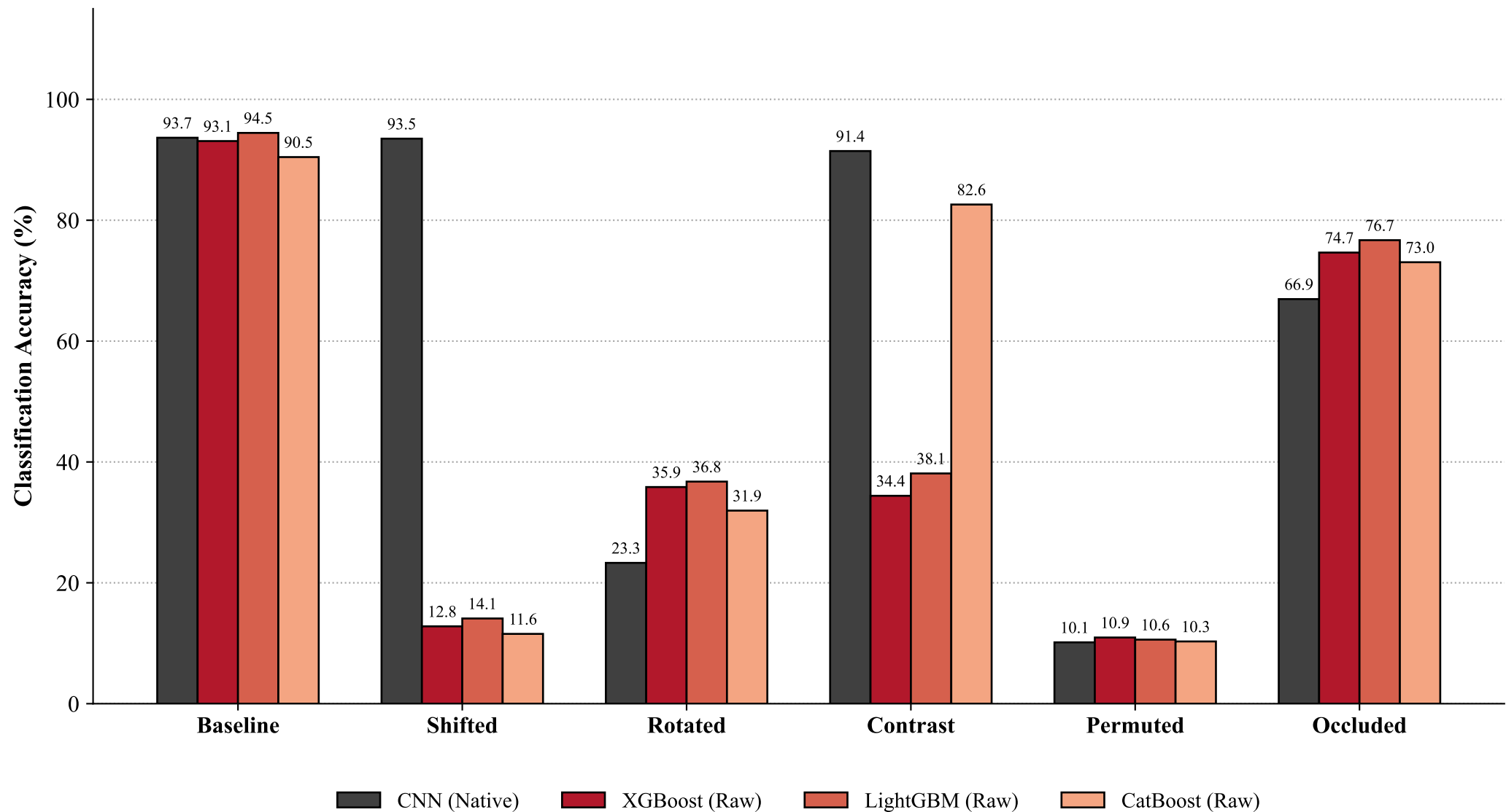
Native CNN vs. Raw Tabular GBDTs
